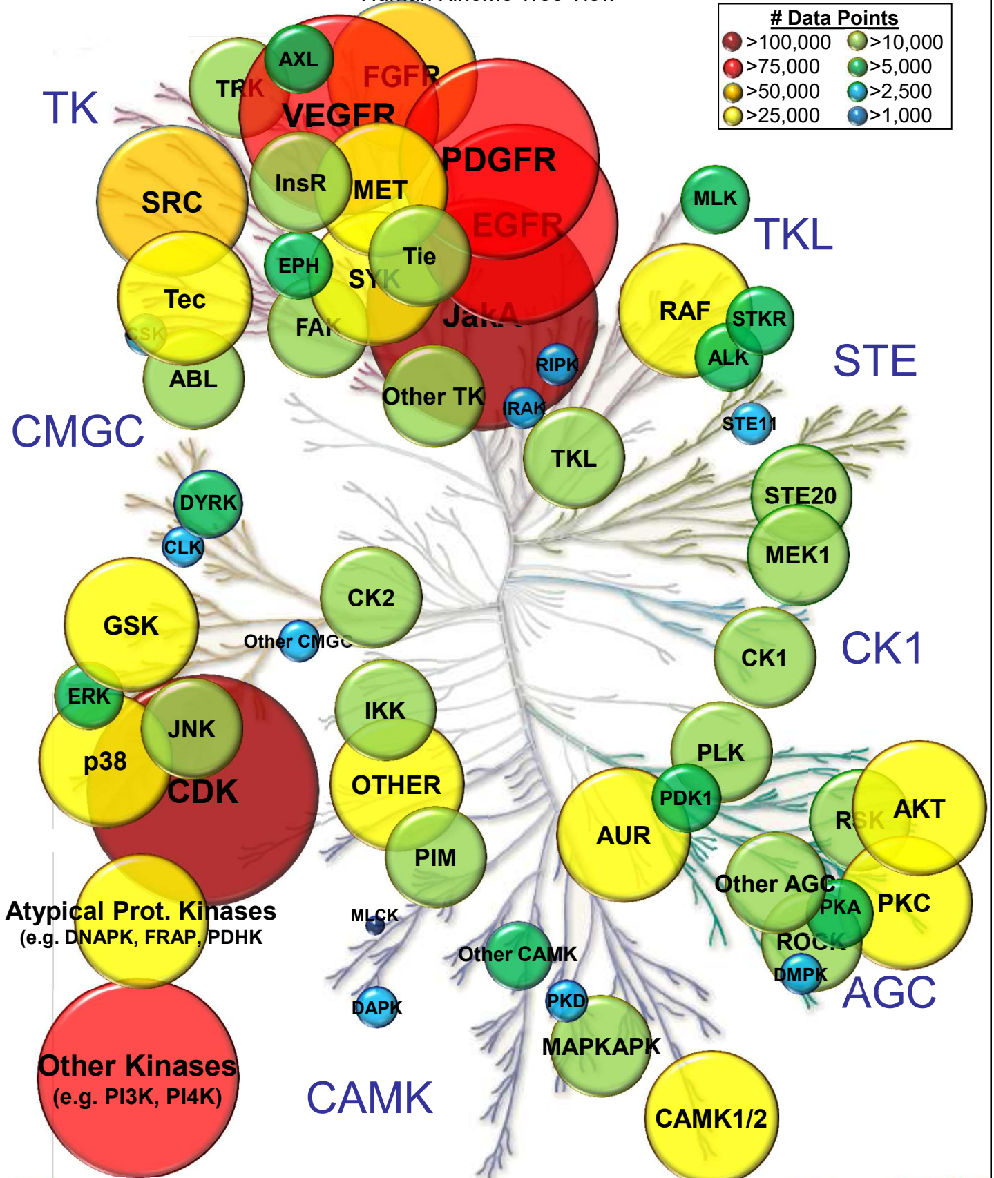
Human Kinome Tree View
